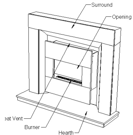
Perspective view
